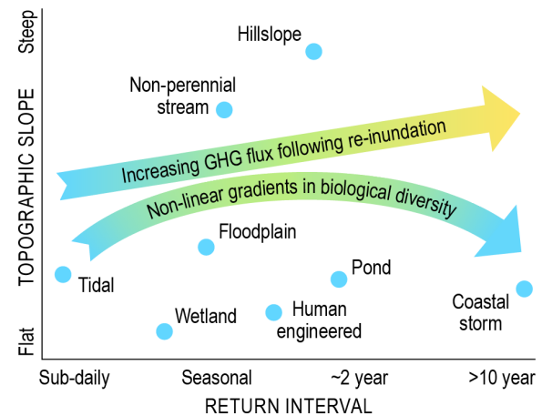
Figure 13. We encourage unifying conceptual models of VIEs based on hypotheses linked to continuous environmental axes, across which these systems can be studied without regard for what system names may be attached to a given studied place and time. In our proposed conceptual model, two key axes are the topographic slope and inundation return interval. Points represent approximate locations of where each VIE type may lie. Each VIE type spans a range of slopes and inundation return intervals, but we do not define these ranges as the conceptual model is based on how study systems fall across the environmental space represented here, rather than within specific nomenclature. Two priority research directions are greenhouse gas (GHG) fluxes and biological diversity, and the arrows represent possible hypotheses that could be evaluated with cross-VIE studies. We propose that knowledge and models that are transferable across VIEs can be achieved through evaluation of such hypotheses across broad ranges in the slope and return interval. Credit: Nathan Johnson.
