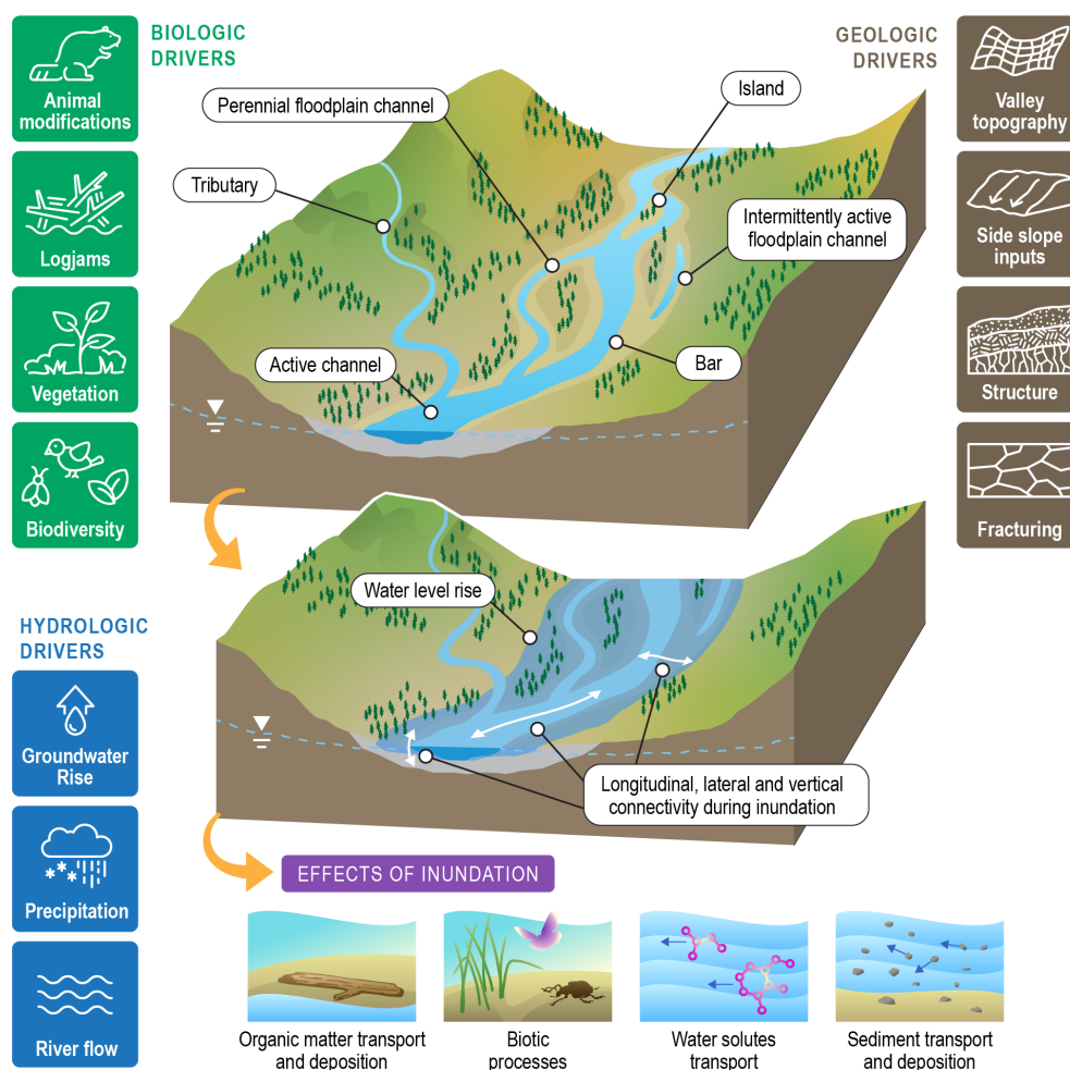
Figure 5. Conceptual model of variable inundation in floodplain and parafluvial systems. Across floodplains and parafluvial zones a suite of biological, hydrologic, and geologic factors drive inundation regimes in terms of spatiotemporal duration, timing, depth, flow rate, etc. These systems include diverse subsystems, as summarized in the top panel. Rising water levels, due to one or more drivers, can inundate these subsystems, as shown in the middle section, resulting in a variety of biogeochemical, ecological, and physical effects (bottom sub-panels). Credit: Nathan Johnson.
