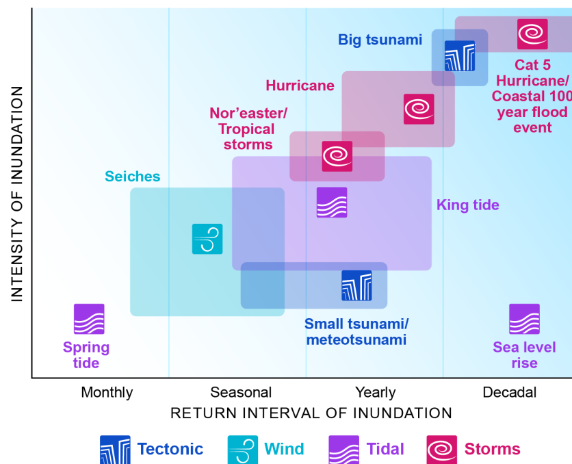
Figure 8. Coastal VIEs experience inundation events with different frequencies and intensities. Some events occur rarely but are of very high intensity (category 5 hurricanes; large tsunamis), increasing the area of inundation and affecting areas that seldom experience inundation. The impacted systems are often less adapted to inundation, increasing the extent of destruction or reorganization of the system. Other events occur more regularly and/or are lower in intensity (spring tide, seiches), leading to less extensive inundation and impacting coastal systems that are more adapted to inundation. Credit: Nathan Johnson.
