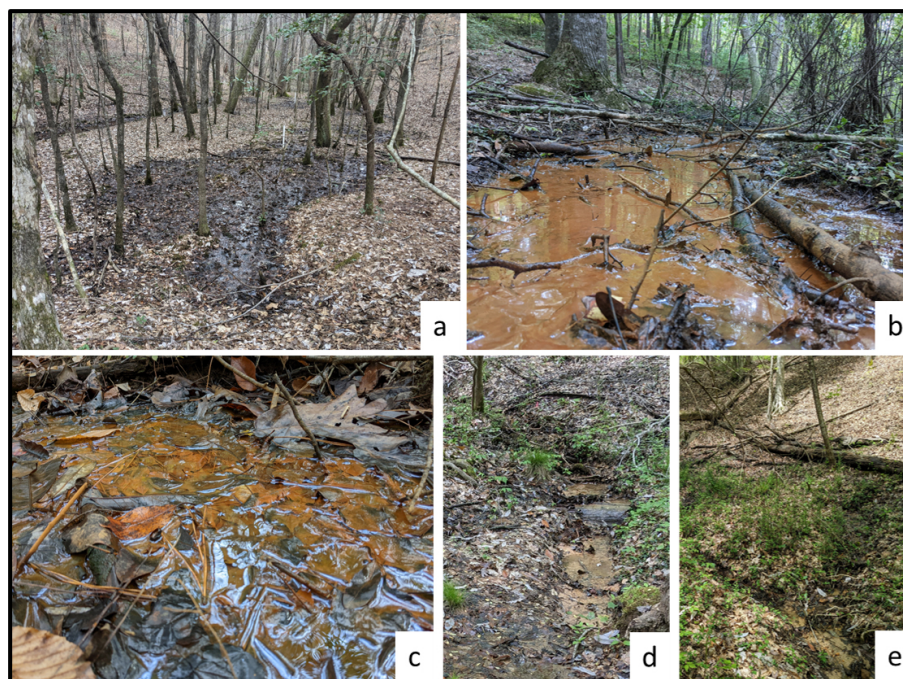
Figure 3. Examples of variable inundation along hillslopes: (a) looking downslope at an inundated slope, (b) ponding with no flow due to microtopography, (c) sheet wash with directional flow across the surface of a hillslope, (d) rill formation with turbid water from erosion, and (e) vegetation community change on a slope due to differences in soil moisture. All photos taken by Corianne Tatariw at Tanglewood Forest, Alabama.
