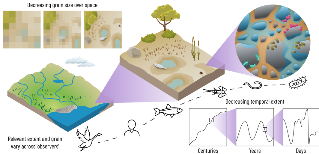
Figure 11. Variable inundation can be observed at different spatiotemporal granularities and extents. Upper left: granularity is based on the resolution of observations in space or time. Lower right: extent is based on the cumulative breadth of observations in space or time. Middle illustrations: granularity and extent of observations are often correlated, such as barely resolving individual trees when extent spans a watershed and resolving individual microbes when extent spans a few soil particles. A given beholder observes variable inundation at a given scale and will, in turn, make changes to behavior, physiology, and/or aspects of life history. For example, migratory waterfowl select habitats based on the inundation state as they move across watersheds, humans plan cities based on regional patterns, fish move across stream reaches based on the continuity of inundation, macroinvertebrates lay eggs on individual rocks based on the inundation state, nematodes experience variable inundation as they move through porous media, and soil microbes separated by micrometers likely experience vastly different inundation dynamics linked to water films on soil particles. Credit: Nathan Johnson.
