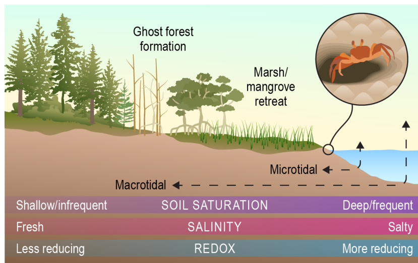
Figure 9. Conceptual model of variable inundation in tidal systems. Tidally driven coastal zones span sediments exposed at low tide to marshes and coastal forests inundated at high tide. This lateral gradient of tidal exposure across micro- to macrotidal systems (dashed black lines) alters physical (e.g., particle deposition), biological (e.g., species composition), and chemical (e.g., nutrient transformations) factors. Organisms can impact conditions along the gradient, such as flow path alteration by crab burrowing. Credit: Nathan Johnson.
