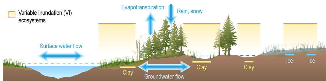
Figure 6. Conceptual model of variable inundation in wetland systems. Different wetland types are influenced and shaped by variable inundation. The absence and presence of surface water is driven by (e.g., seasonally) changing water supply and the hydrologic function of the wetland in the landscape. Sediment characteristics (e.g., clay or ice) and topographic positions of wetlands in the landscape influence water loss to infiltration or gain from groundwater. Credit: Nathan Johnson.
