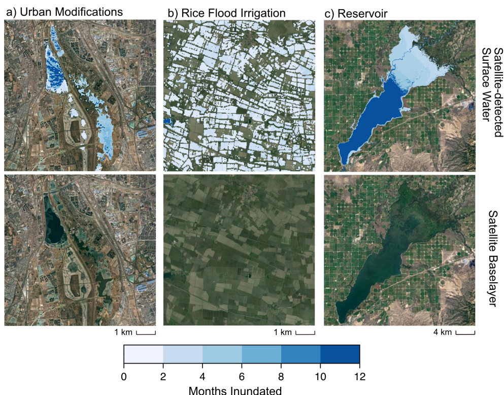
Figure 10. Examples of human-engineered variably inundated ecosystems: (a) Yongding River in Beijing, China; (b) paddy rice fields in northern Italy; (c) American Falls Reservoir on the Snake River in Idaho, United States. These three examples emphasize significant variation in the degree of variable inundation across human-engineered VIEs, with some regions being perennially inundated. Top row: satellite-derived map data on months inundated are derived from the “seasonality” product in the Global Surface Water Mapping Layers v1.4 (Pekel et al., 2016). Credit: Jillian Deines.
