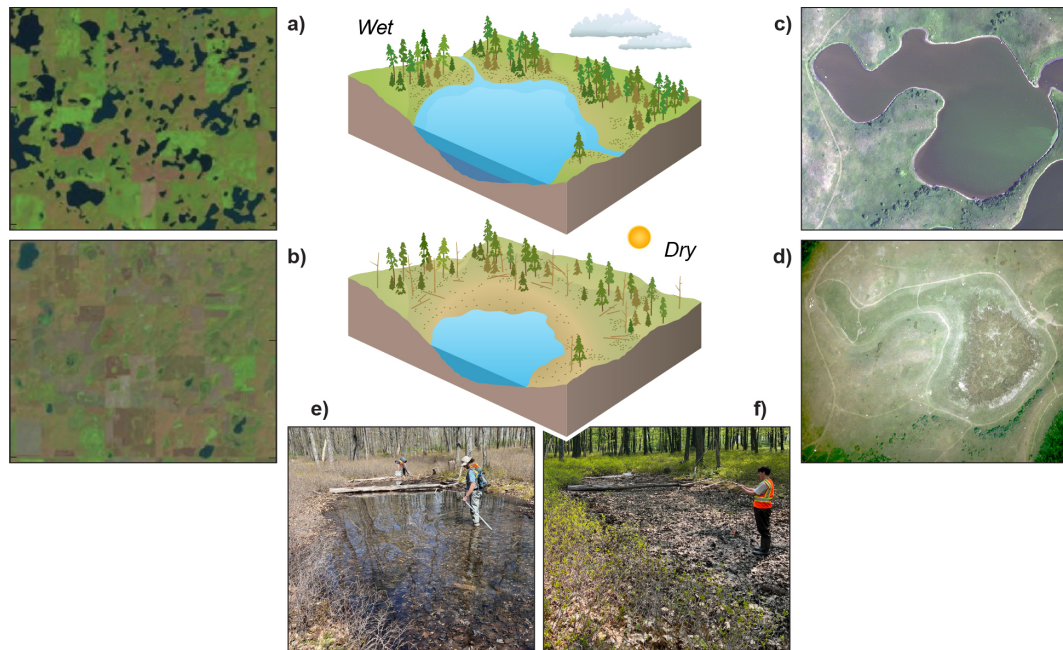
Figure 7. Examples of variable inundation across scales in pond systems. Satellite imagery of the Prairie Pothole Region, North Dakota, USA, illustrating decadal variable inundation at a landscape scale on (a) 2 September 1992 and (b) 23 May 2013 (modified from Anon, 2015) and at the pond scale – aerial imagery of Pond P1, Cottonwood Lake Study Area, North Dakota, on (c) September 2002 and (d) September 1992 (images from the US Geological Survey, 2017). Seasonal changes in a vernal pond in Moshannon State Forest, Pennsylvania, USA, (e) inundated (11 May 2023) and (f) non-inundated (23 May 2023) (Jon N. Sweetman). Conceptual drawings by Nathan Johnson.
