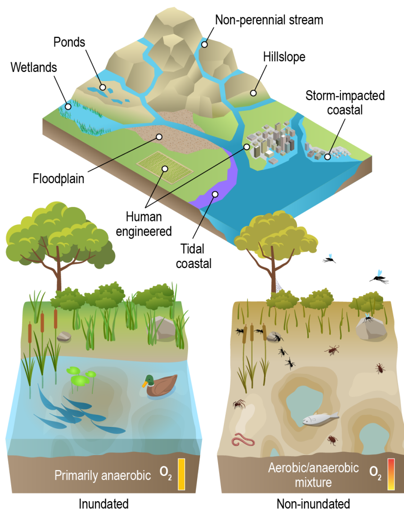
Figure 2. Conceptual overview of where different types of VIEs are often found within watersheds and some common shifts in system states across inundated and non-inundated conditions. VIEs are found in locations from headwaters to coastal environments (top), and the impacts of variable inundation have some consistencies across these diverse landscapes (bottom). Organismal ecology, physiology, and demographics are altered by variable inundation, leading to shifts in community composition. Biogeochemical processes also shift, such as greater gas-phase transport of oxygen into soil/sediment when surface water is lost. A key goal for cross-VIE science is to mechanistically understand variation in the impacts of variable inundation across multi-dimensional environmental space. Credit: Nathan Johnson.
