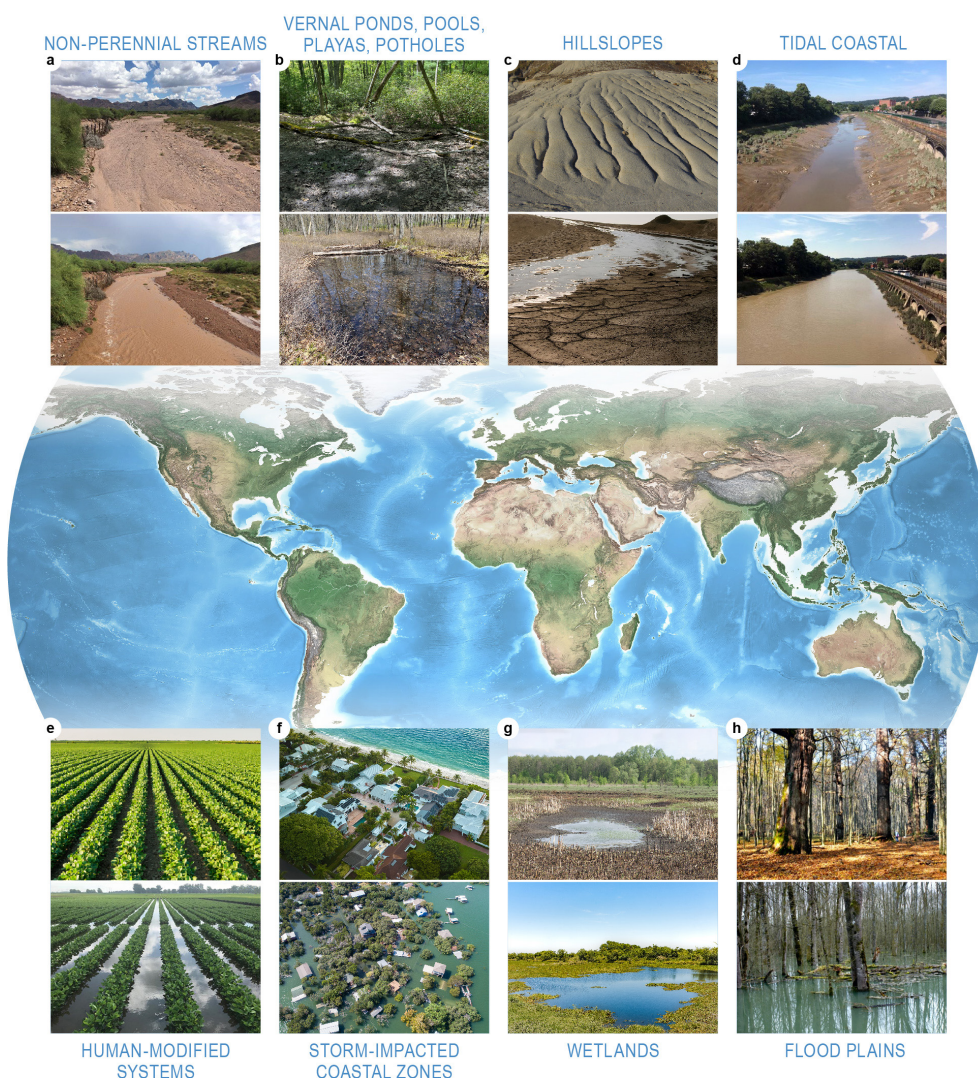
Figure 1. Variably inundated ecosystems (VIEs) span numerous ecosystem types and are globally distributed across Earth's land surface. There are few places across Earth's land surfaces that do not experience variable inundation, which is defined here as the loss/gain of an aqueous barrier between the atmosphere and porous media (e.g., soil) that inhibits gas-phase transport. Due to global changes in the dynamics of variable inundation, there is a need to integrate knowledge into models that are predictive across VIEs. This will require intentionally studying VIEs together to understand how the details of any given VIE modulate the impacts of variable inundation. Credit: Nathan Johnson. There are several photos, used with permission, from different sources as follows: (a) Sullivan et al. (2019); (b) Jon Sweetman, co-author; (c) Shutterstock; (d) WeirdBristol (2018); (central global image, e, f, g) Shutterstock; and (h) Mikac et al. (2018).
