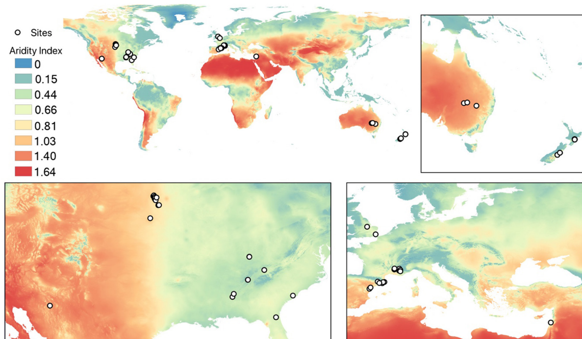
Figure 1. Climatic aridity across the study sites ( n=112 ). Aridity is defined as the ratio between mean annual precipitation and mean annual potential evapotranspiration, using the WorldClim global dataset (Hijmans et al. 2005) (Methods for details).
