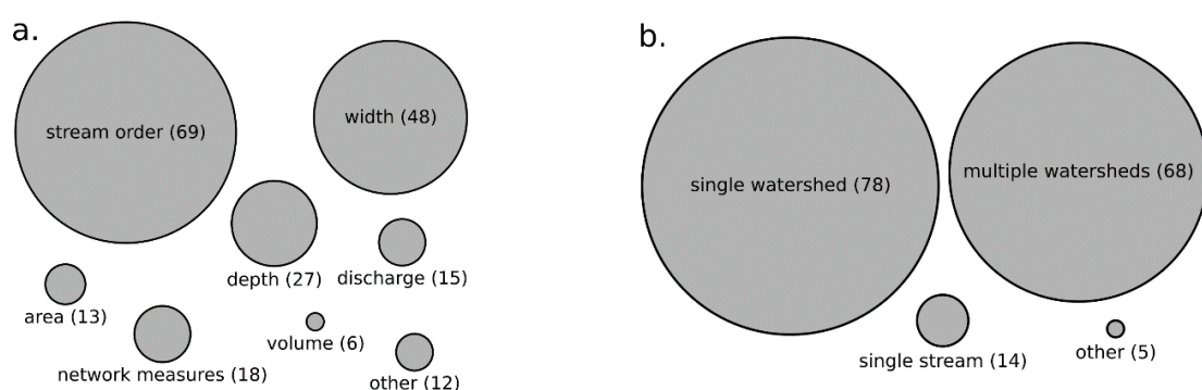
Figure 3. Measures of stream size used to infer biodiversity–stream size relationships (a) Network measures includes measures such as link distance from source, downstream, links magnitude, and several other measures. Geographic scale of studies inferring relationships between stream size and biodiversity (b) The category “other” includes continental, global, and single reach.
